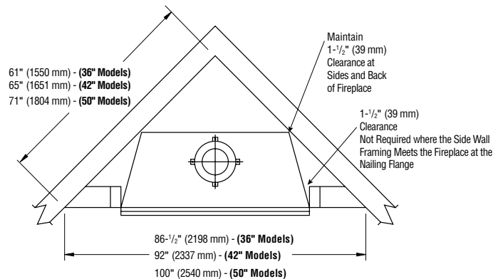
Figure 5 - Corner Installation
