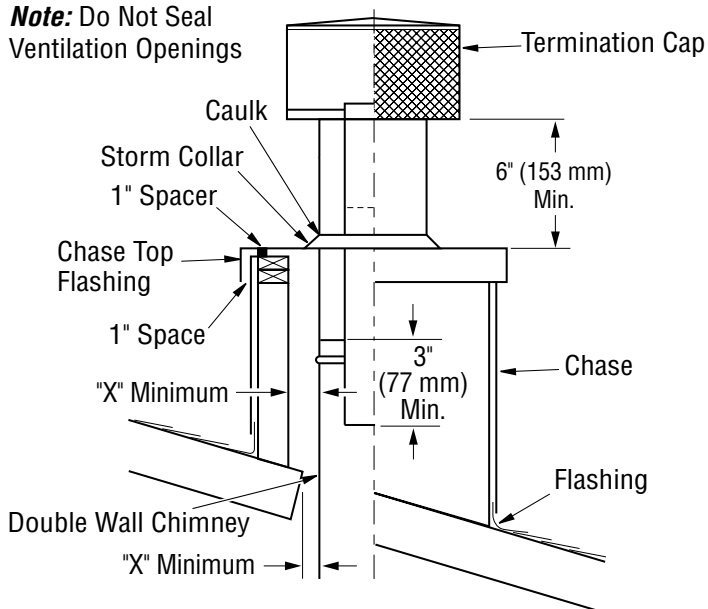
Figure 29 - Chase Installation
