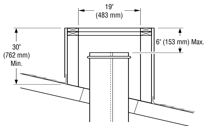
Figure 21 - Constructing Chase
