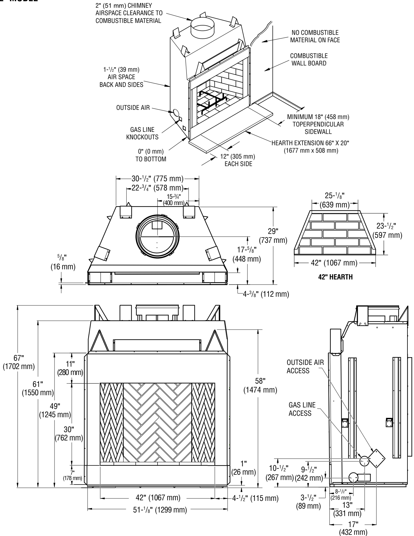
Figure 2 - 42" Models
