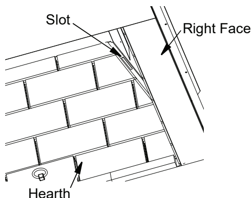
Figure 14 - Slots for Firebrick Walls
