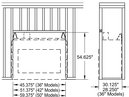
Figure 8 - Framing Dimensions
