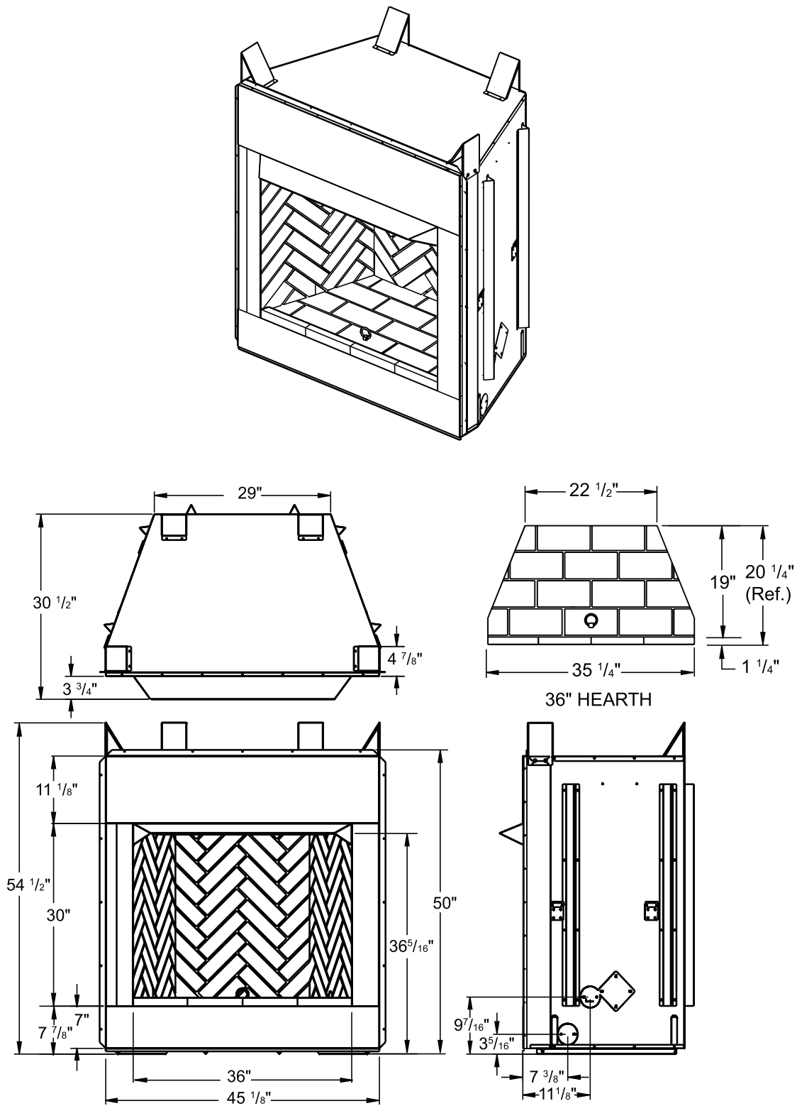
Figure 1 - 36" Models VRT6036RS, VRT6036IS, VRT6036RH, VRT6036IH
