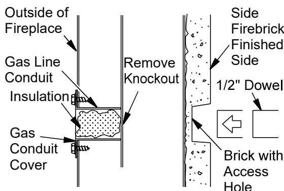
Figure 18 - Gas Line Access
