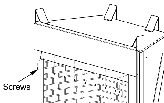
Figure 16 - Screw and Hood Placement
