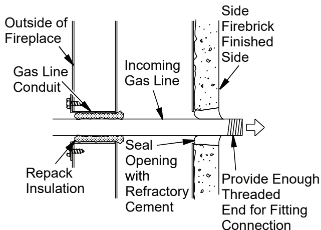
Figure 19 - Gas Line Installation
