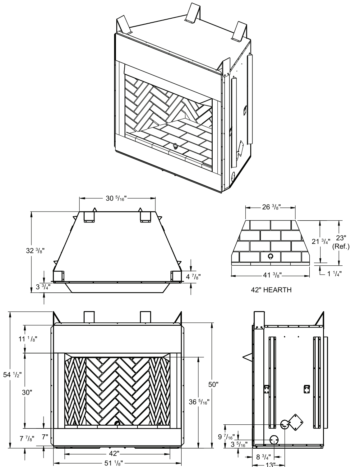
Figure 2 - 42" Models VRT6042RS, VRT6042IS, VRT6042RH, VRT6042IH
