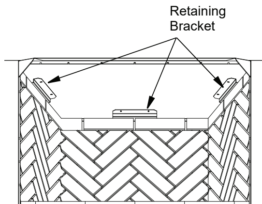
Figure 15 - Installing Side Walls
