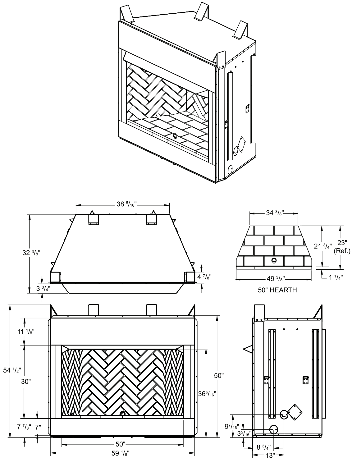
Figure 3 - 50" Models VRT6050RS, VRT6050IS, VRT6050RH, VRT6050IH
