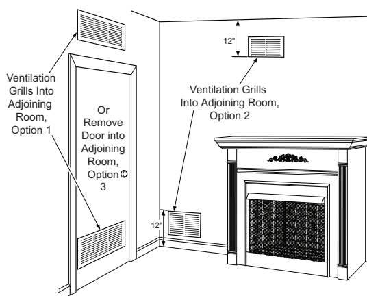
Figure 4 - Ventilation Air from Inside Building
