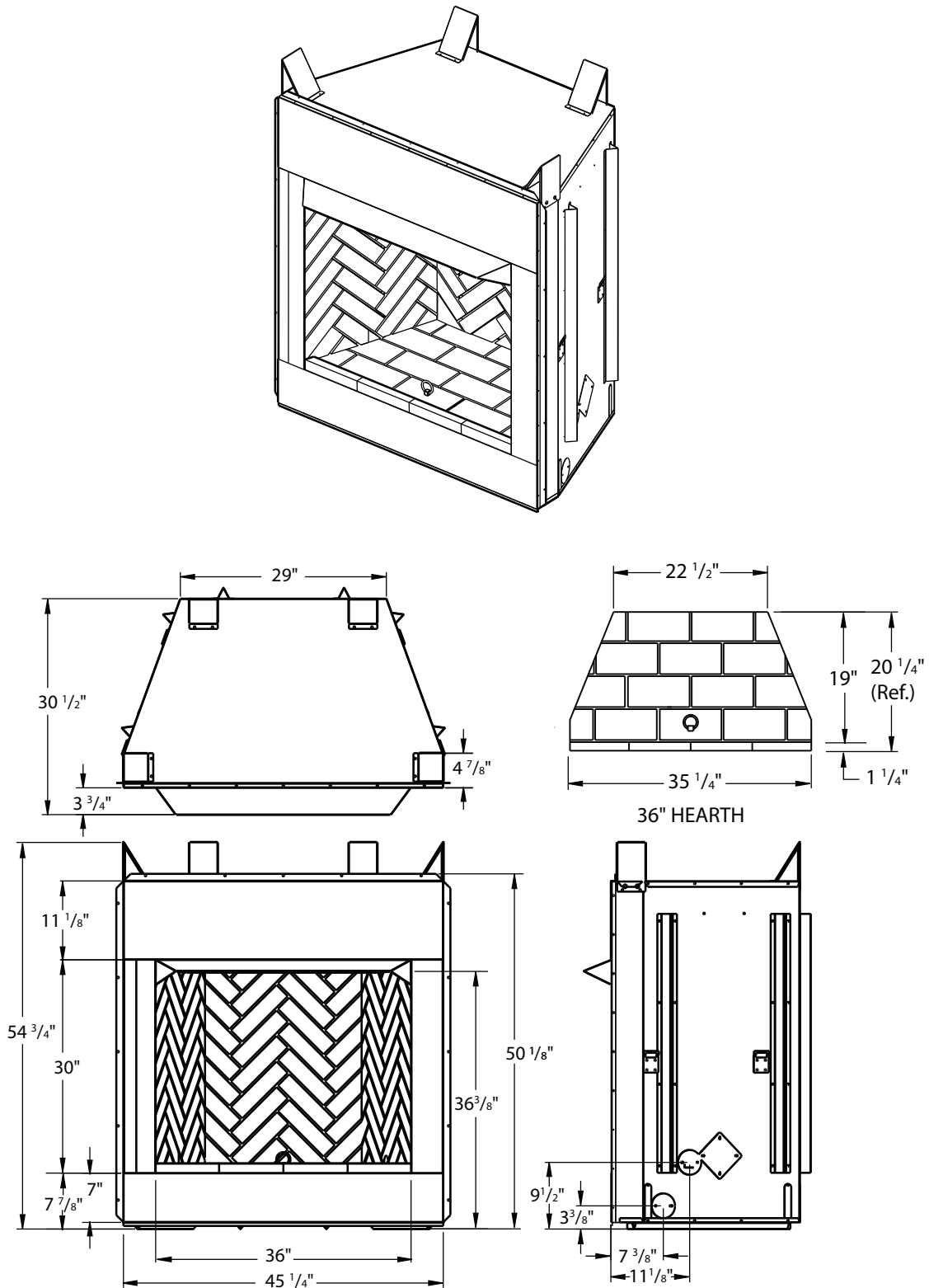
Figure 1 - 36" Models VRT4536WS and VRT4536WH (Picture may vary from actual fireplace)
