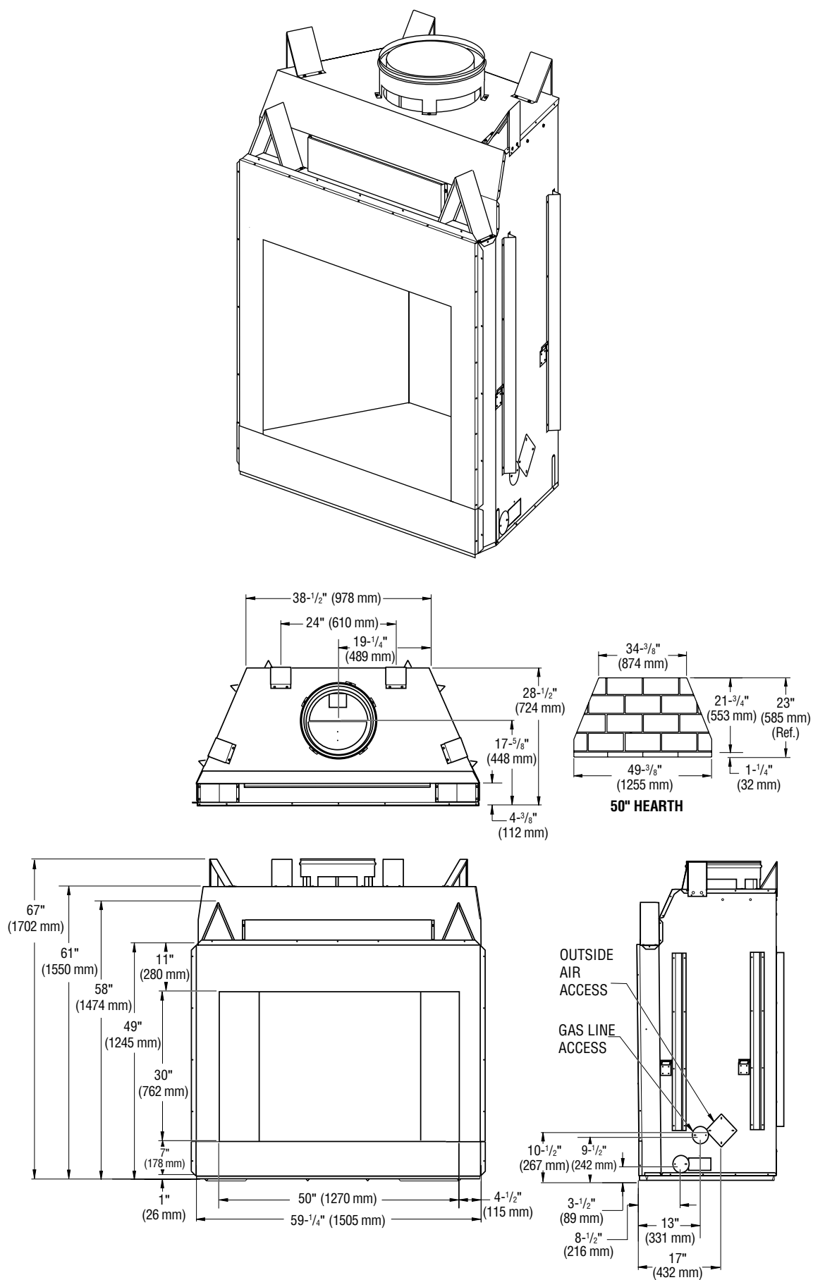
Figure 3 - 50" Model Oracle50
