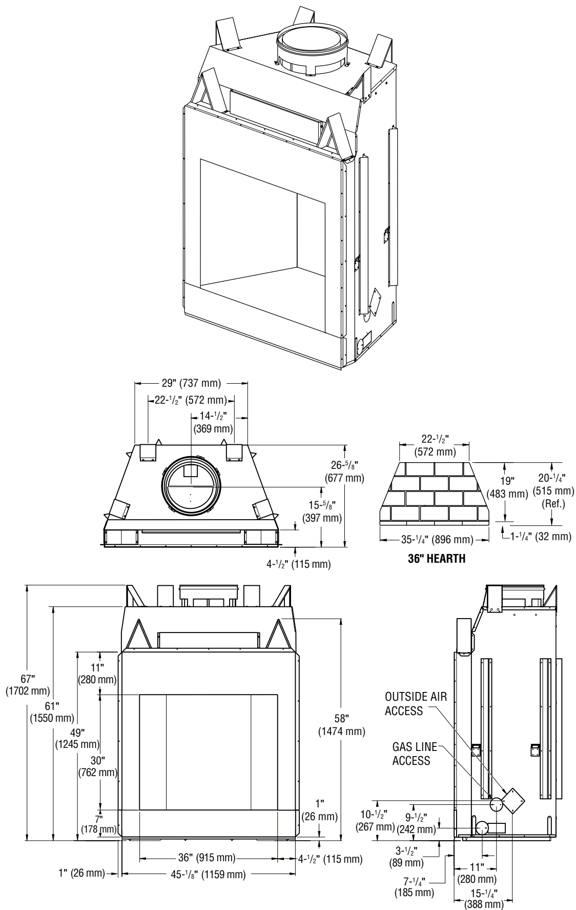
Figure 1 - 36" Model Oracle36
