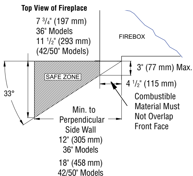
Figure 7 - Mantel Clearances to Combustible Material
