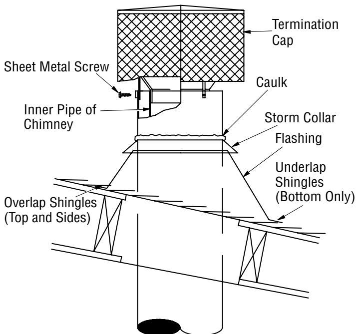
Figure 30 - Non-Chase Installation
