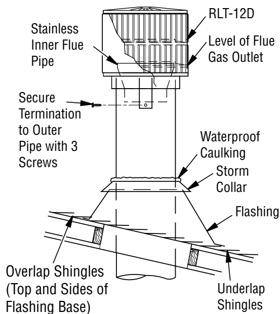
Figure 18 - Termination
