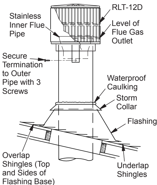
Figure 17 - Termination
