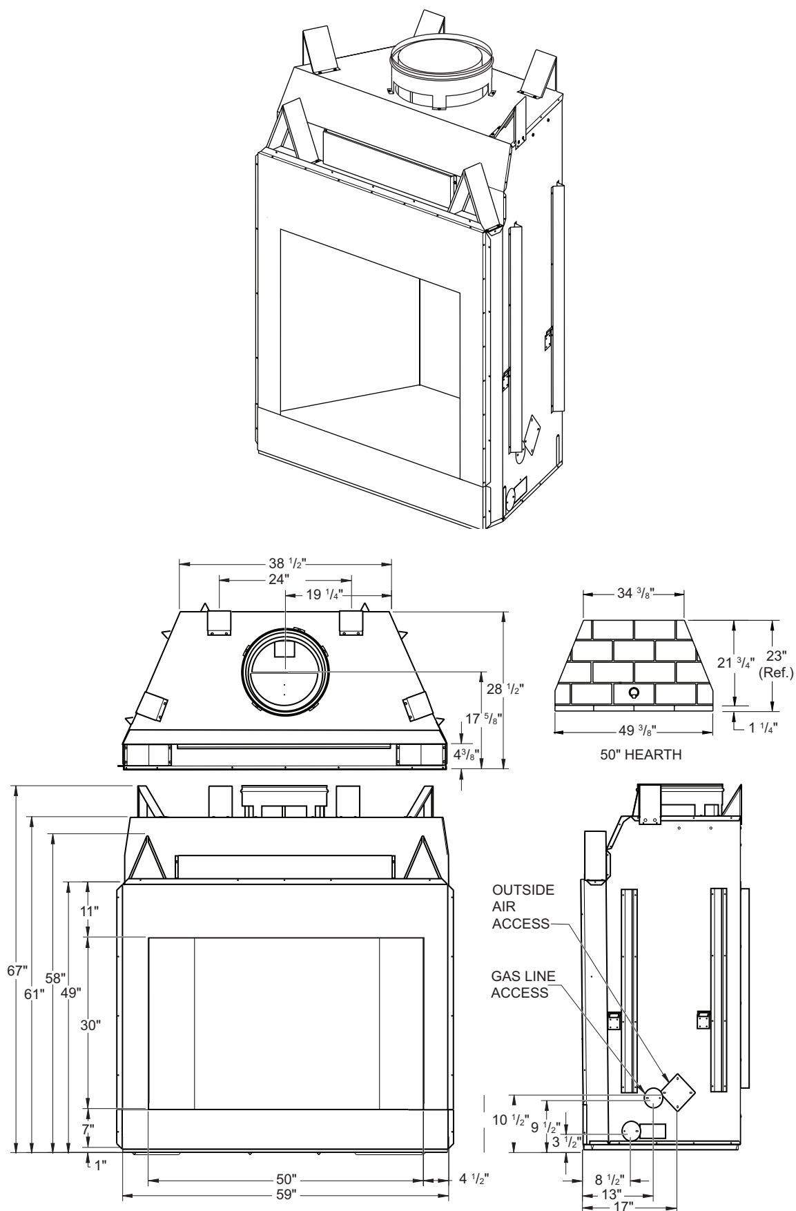
Figure 2 - 50" Model Oracle Cat 50
