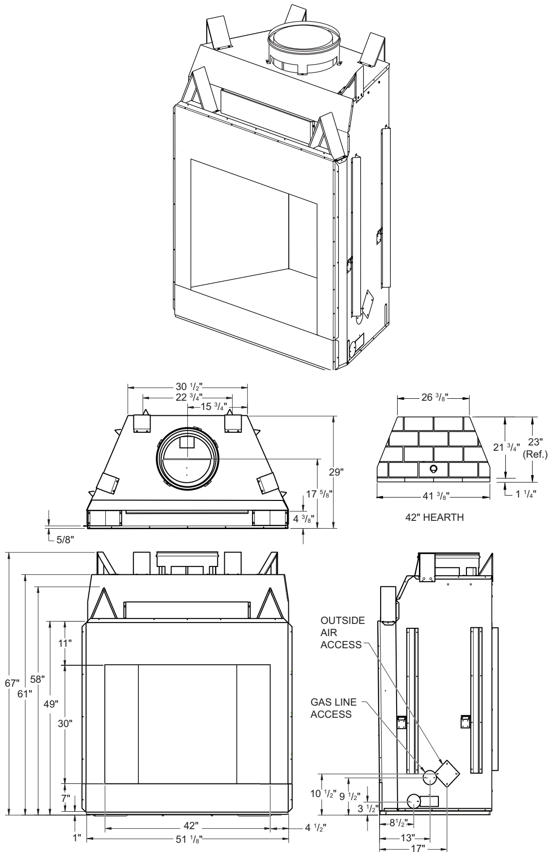
Figure 1 - 42" Model Oracle Cat 42
