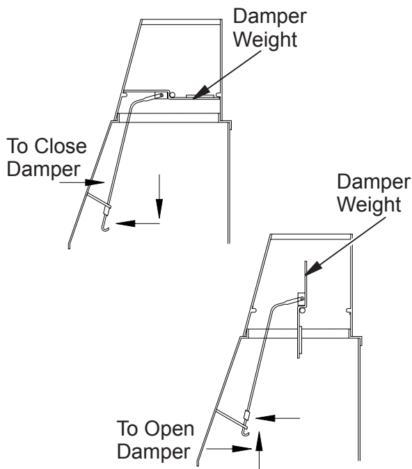
Figure 35 - Operating Damper Handle
