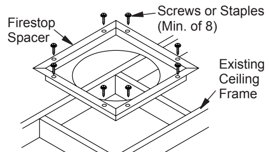
Figure 13 - Firestop Spacer with Attic Space Above Ceiling
