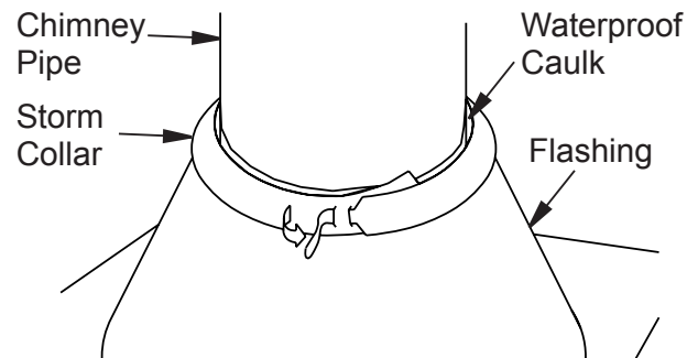
Figure 16 - Storm Collar
