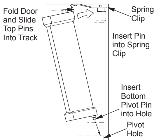
Figure 32 - Installing Bi-Fold Doors
