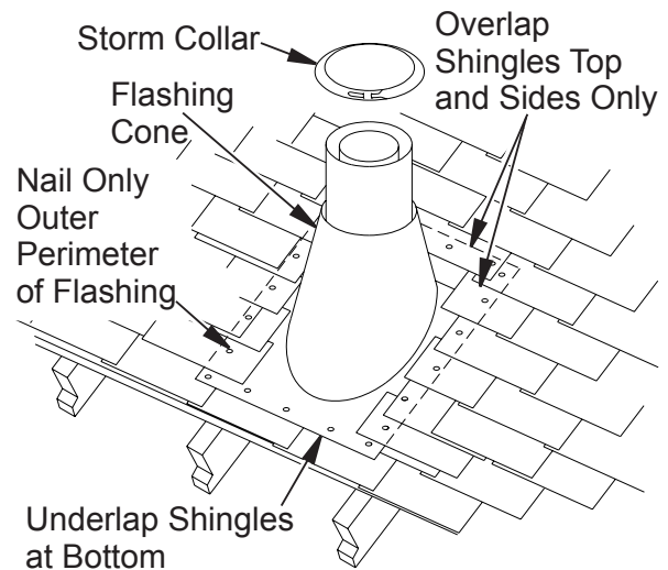
Figure 15 - Flashing Installation
