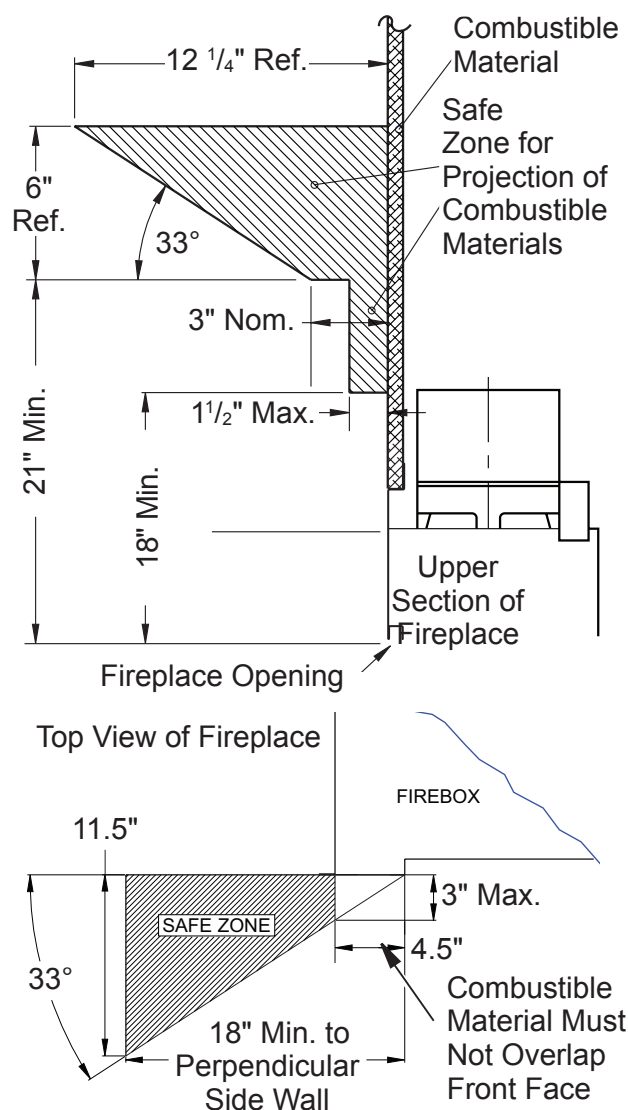
Figure 6 - Mantel Clearances to Combustible Material
