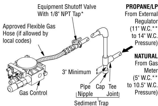
Figure 12 - Gas Connection
