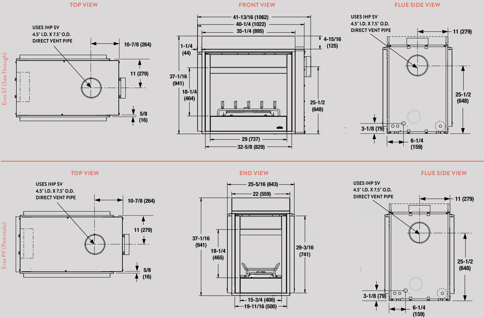
LIBRA MULTI-VIEW FIREPLACE EFFICIENCIES — Listed to ANSI Z21.88 as a gas fireplace heater
