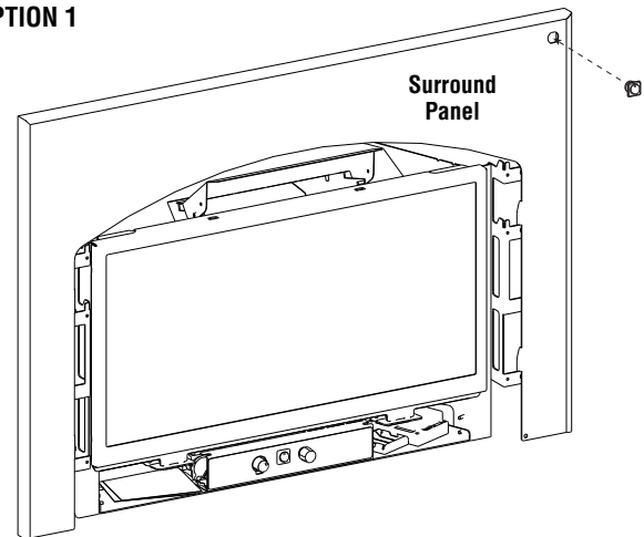
Figure 16 - Burner ON/OFF Switch On Surround
