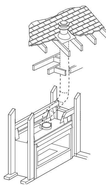
Offset Venting
