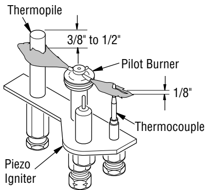
Figure 27 - Pilot Assembly
