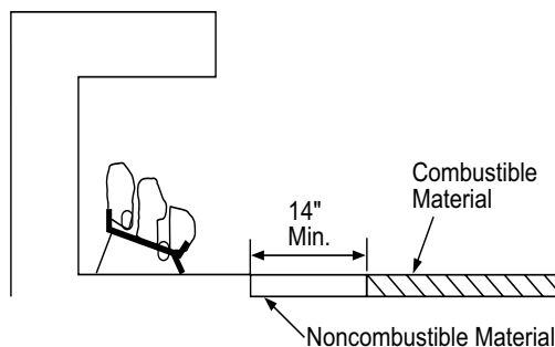
Figure 6 - Minimum Fireplace Clearances If Installed at Floor Level
