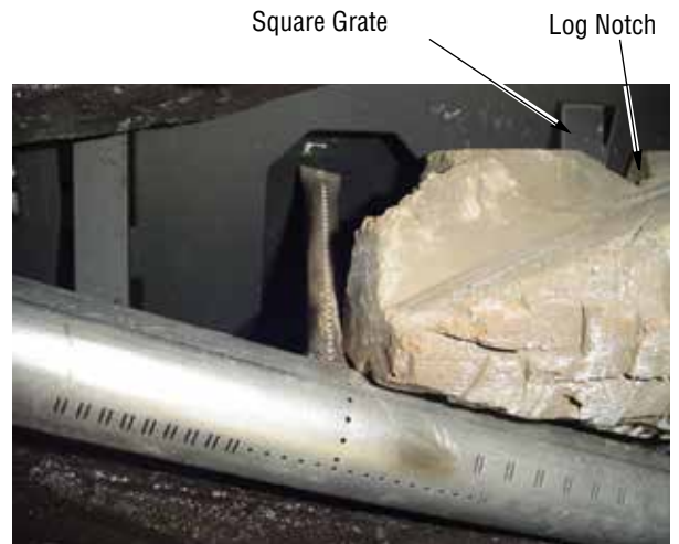
Figure 20B - Installing Charred Log Top Side View
