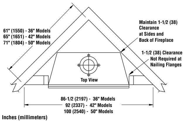
Corner Framing Dimensions
