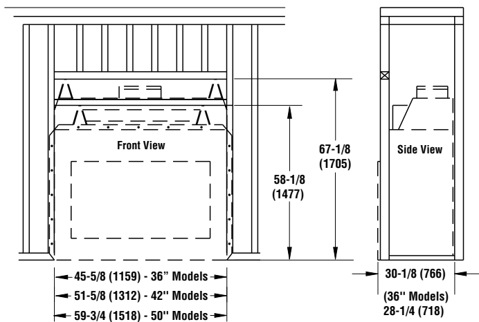
Parallel Framing Dimensions
