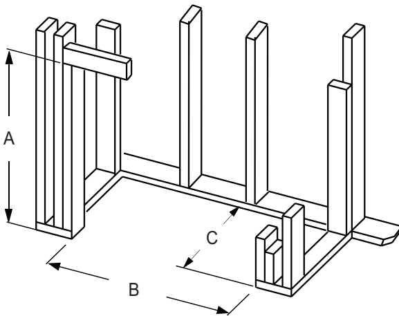
Framing Dimensions
