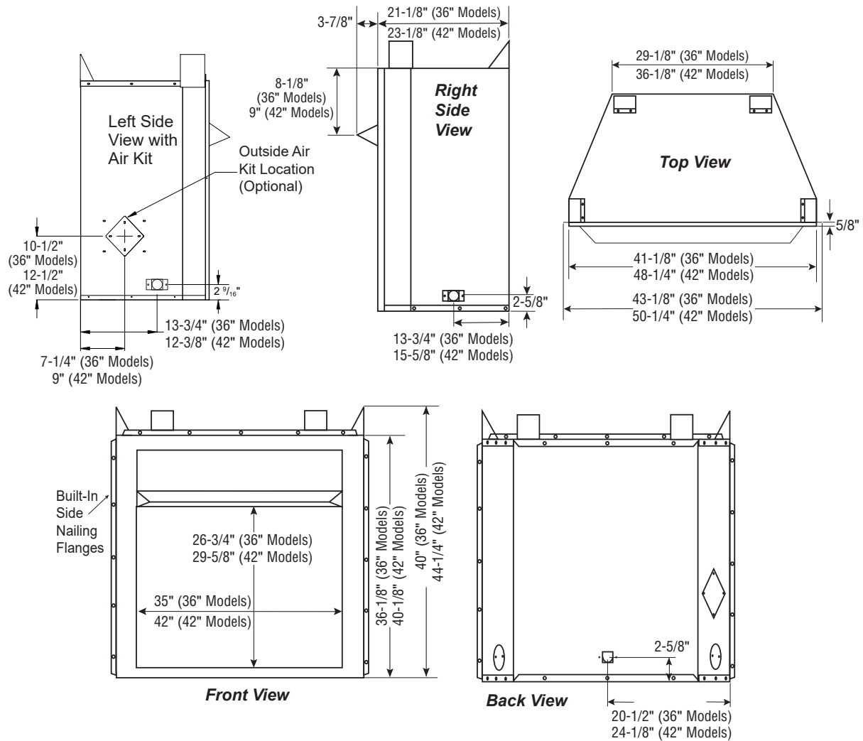
Fireplace Dimensions
