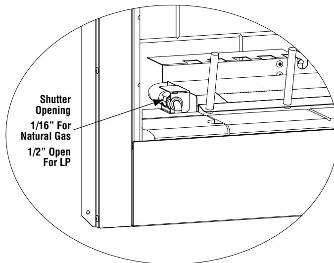
Figure 18 - Burner Air Shutter Settings
