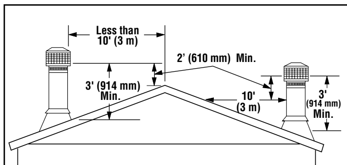
Figure 1 - Chimney Height Requirements
