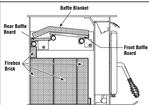
Figure 4 - Side Cut-A-Way View of Firebox
