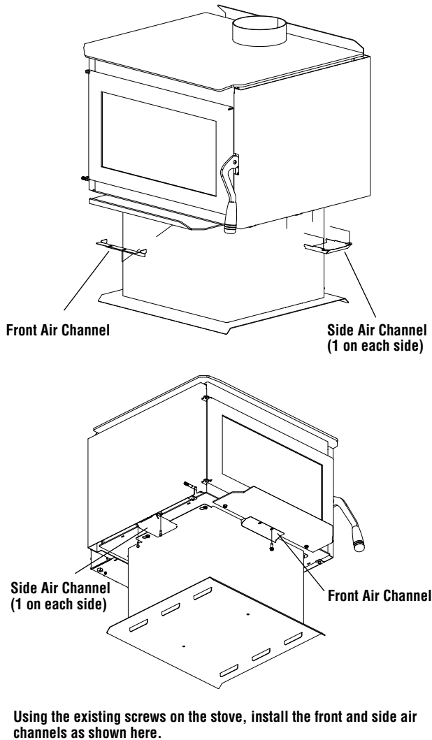
Figure 12 - Install Front and Side Air Channels
