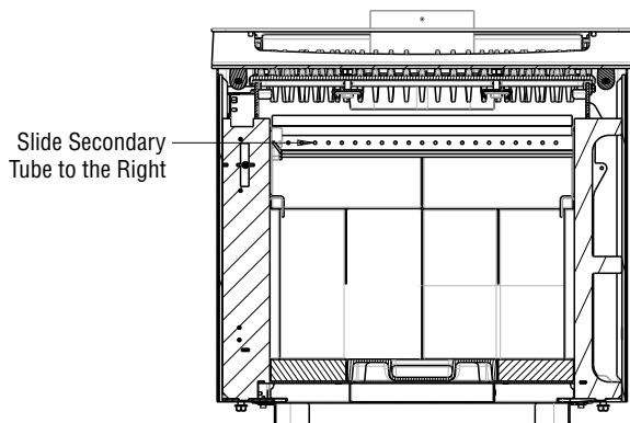
Figure 25 - Secondary Air Tubes
