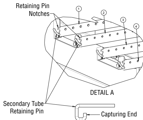
Figure 26 - Secondary Air Tube Retainers
