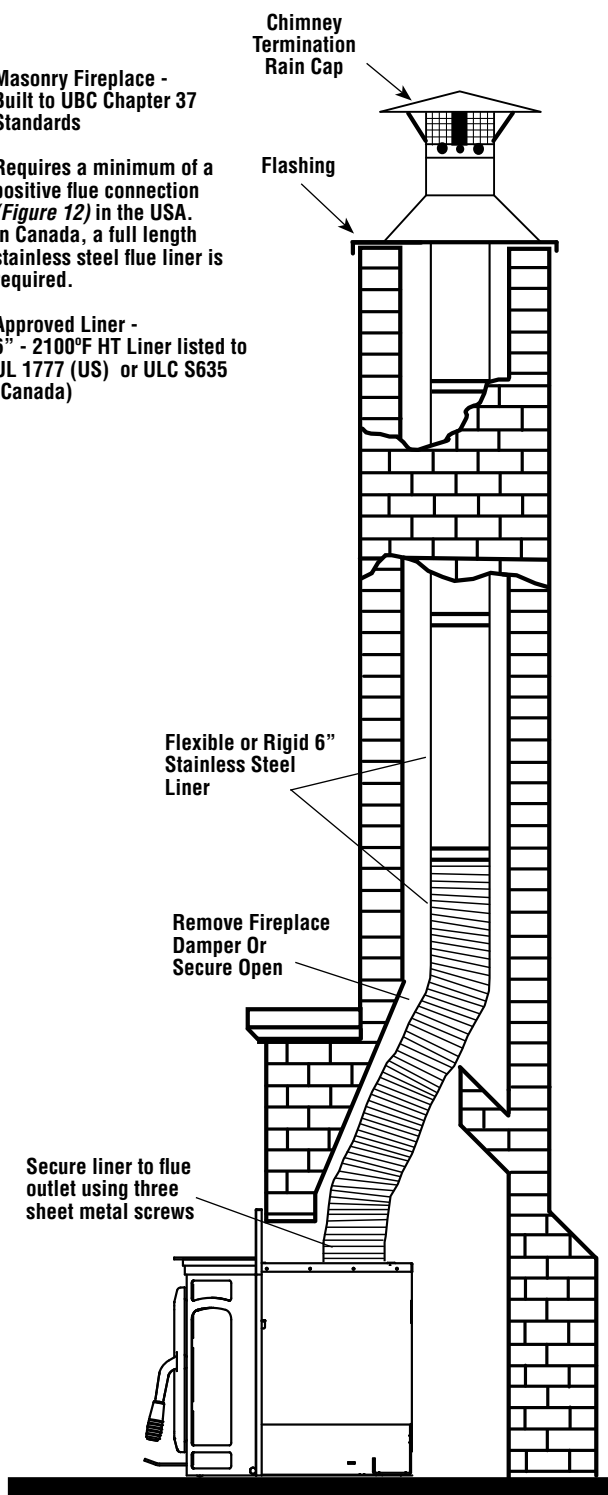
Figure 16 - Typical Installation - Masonry Fireplace
