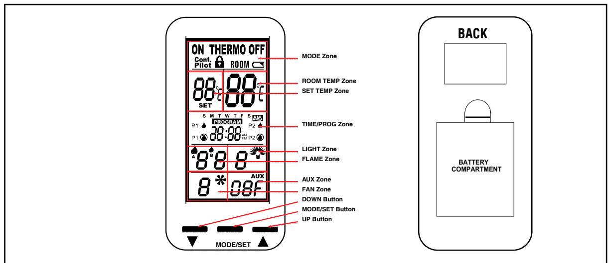
Figure 40 - Remote Control
