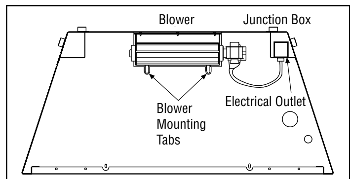
Figure 45 - Blower Installation
