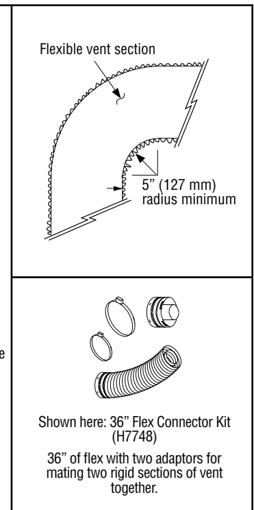
Figure 33 - Flexible Vent
