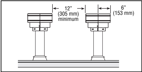
Figure 3 - Multiple Terminations
