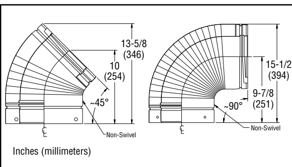
Figure 20 - Elbow Dimensions
