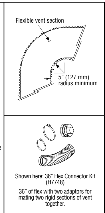
Figure 33 - Flexible Vent
