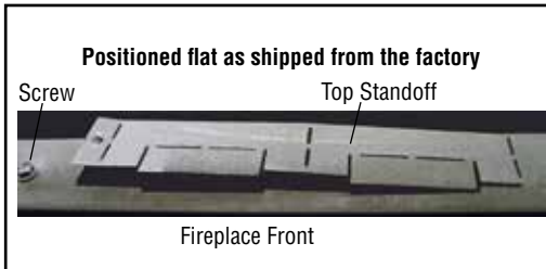
Figure 7 - Unassembled standoff
