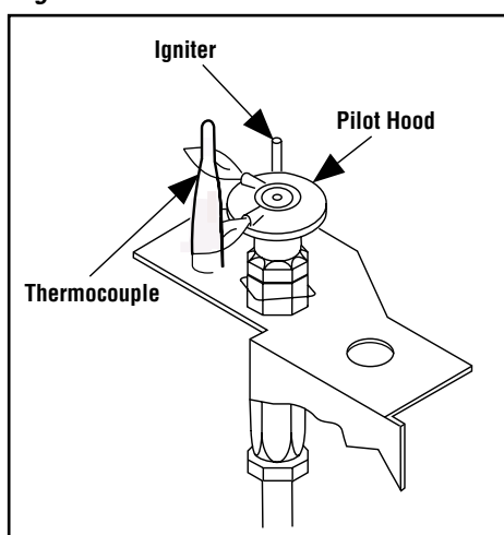
Figure 39 - Electronic Pilot
