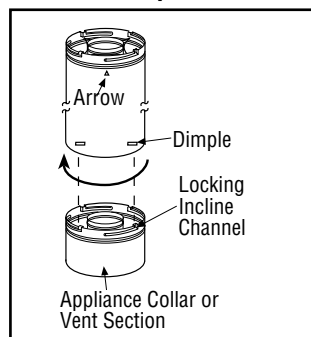
Figure 18 - Connecting vent components
