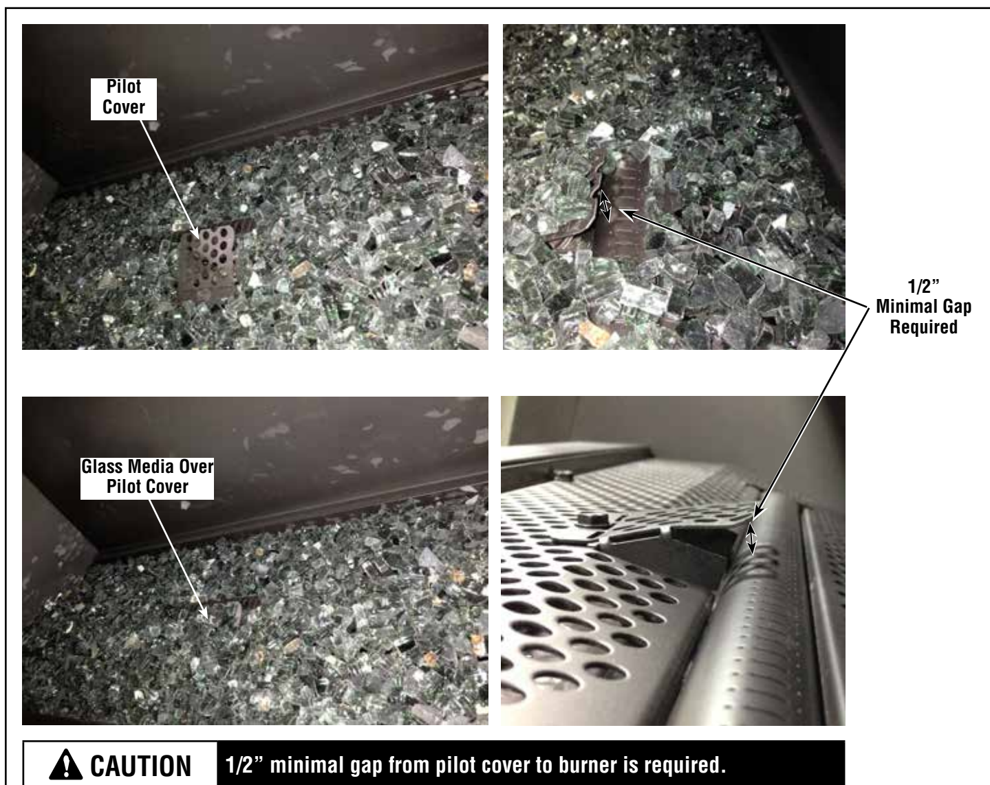
Figure 53 - Removing Sticker and Placing Glass Media Over Pilot Cover.
