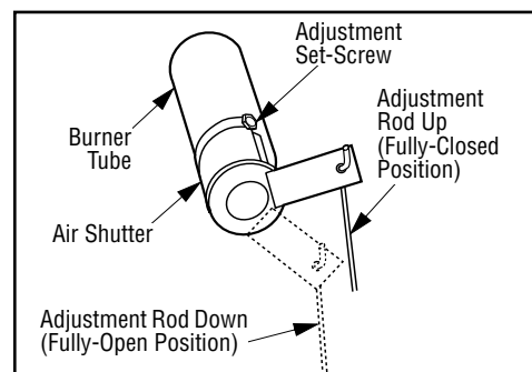
Figure 41 - Air Shutter Adjustment Rod
