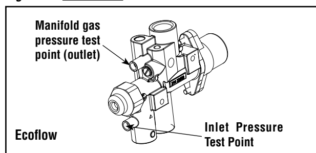
Figure 1 - MANIFOLD Outlet Gas Pressure Test Point
