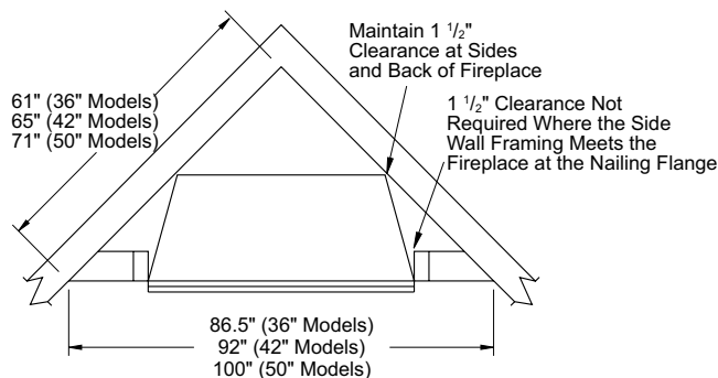
Figure 9 - Corner Installation
