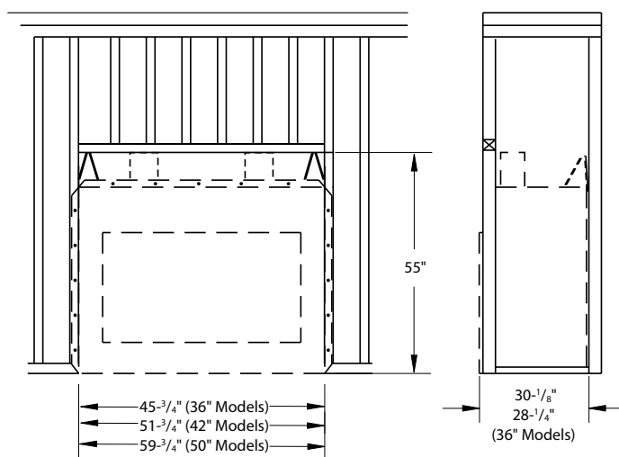
Figure 8 - Framing Dimensions
