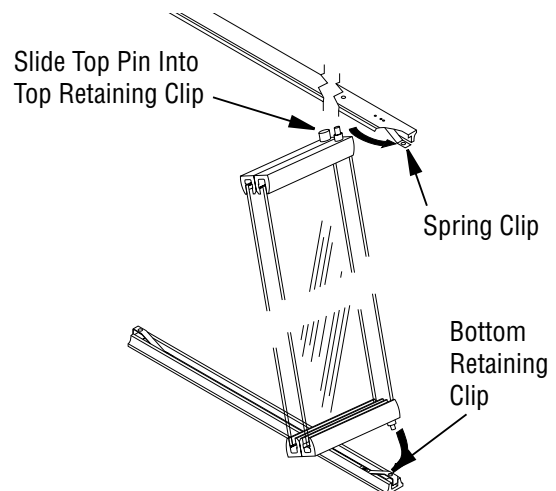
Figure 40 - Installing Doors
