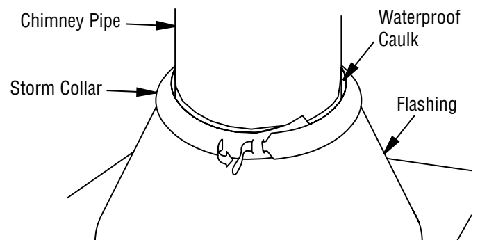
Figure 14 - Storm Collar
