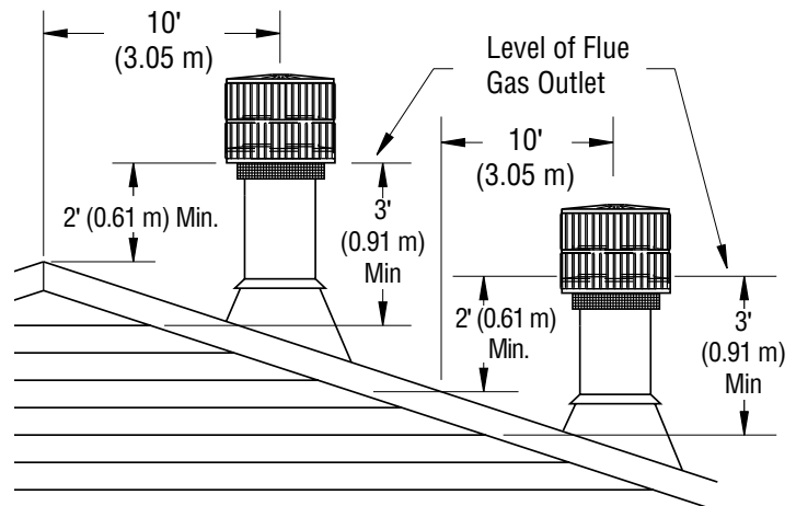
Figure 17 - 10 Foot Rule
