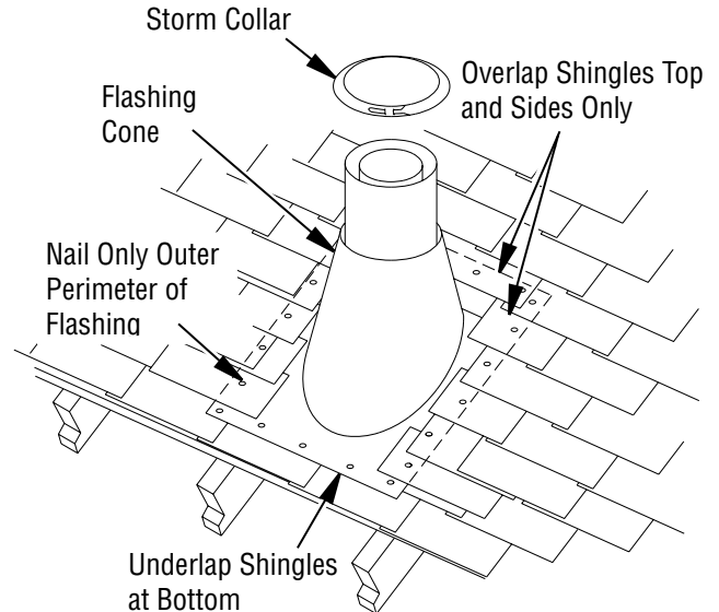
Figure 13 - Flashing Installation
