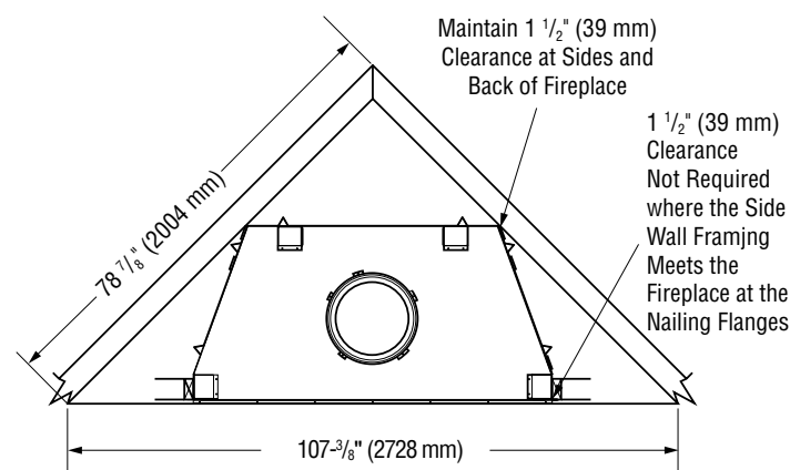
Figure 1 - Framing Dimensions
