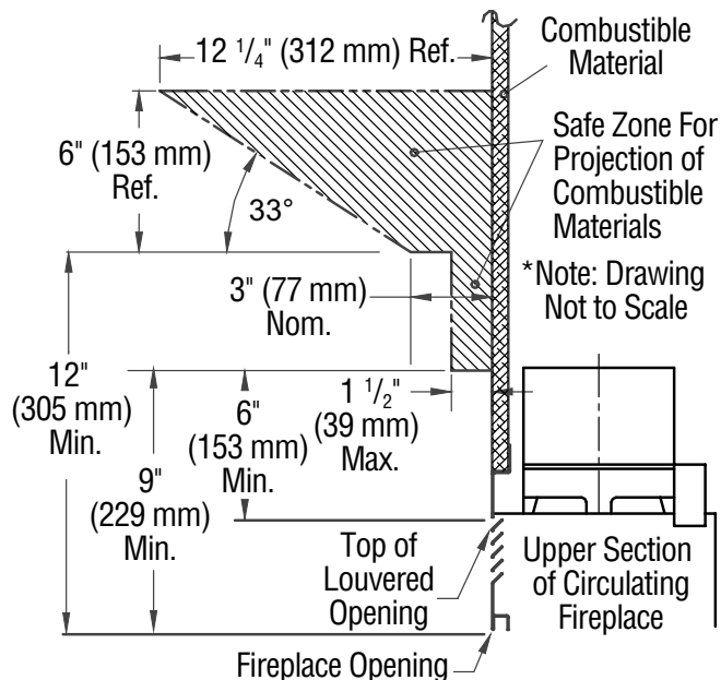
Figure 4 - Mantel Clearances to Combustible Material
