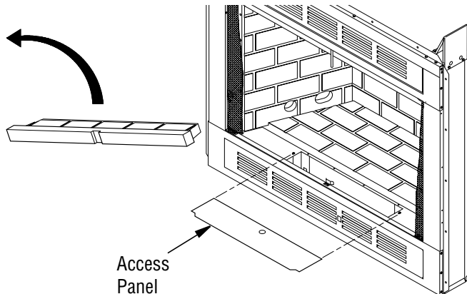
Figure 26 - Locating Access Cover Plate
