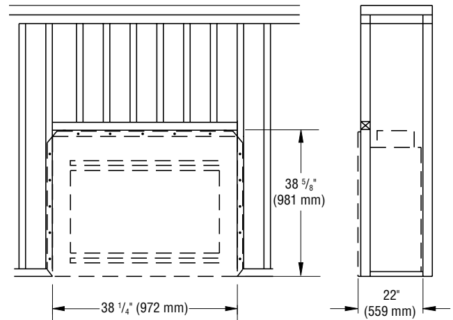
Figure 1 - Framing Dimensions
