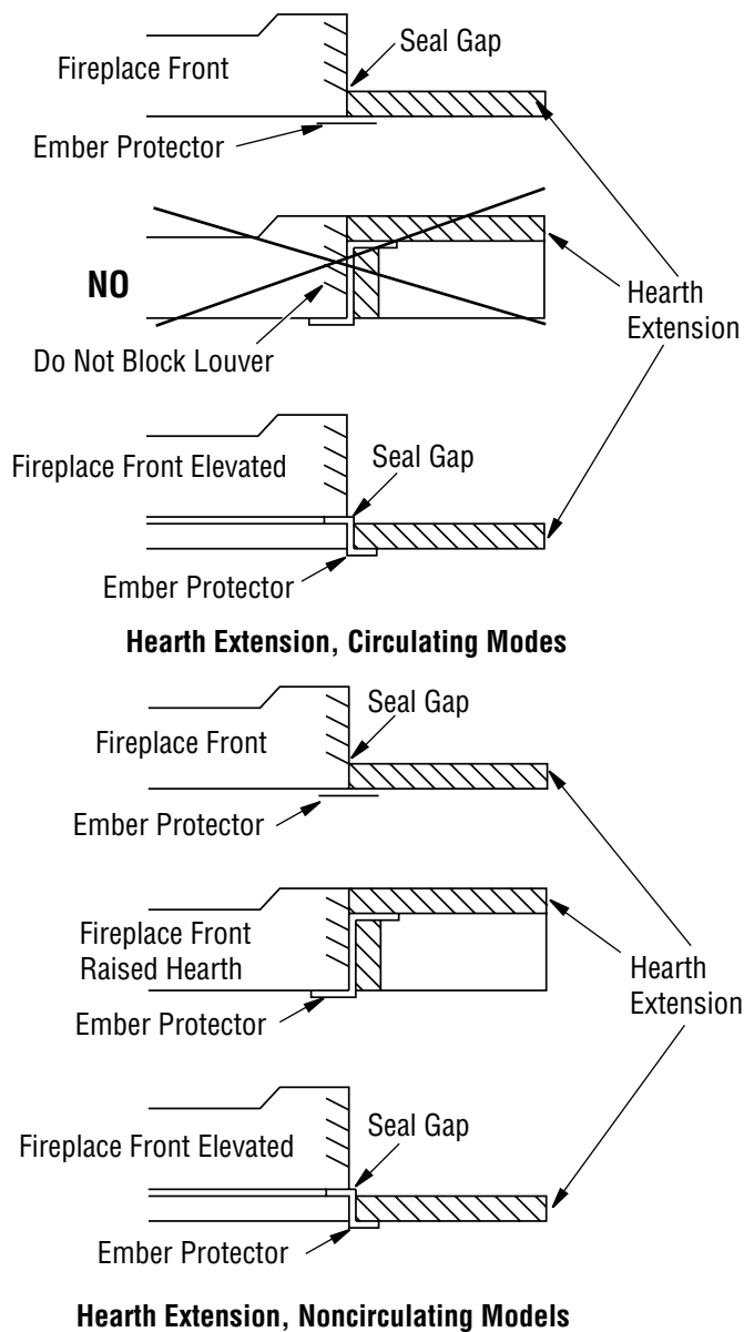
Figure 3 - Hearth Extension
