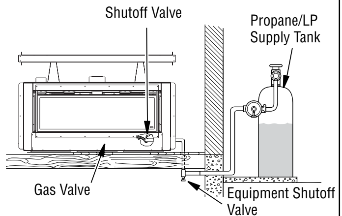
Figure 30 - Checking Gas Joints for Propane/LP Gas Fireplace
