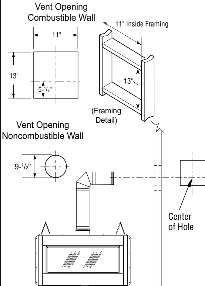
Figure 13 - Vent Opening Requirements
