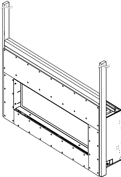
Figure 42 - Non-Combustible Fireboard
