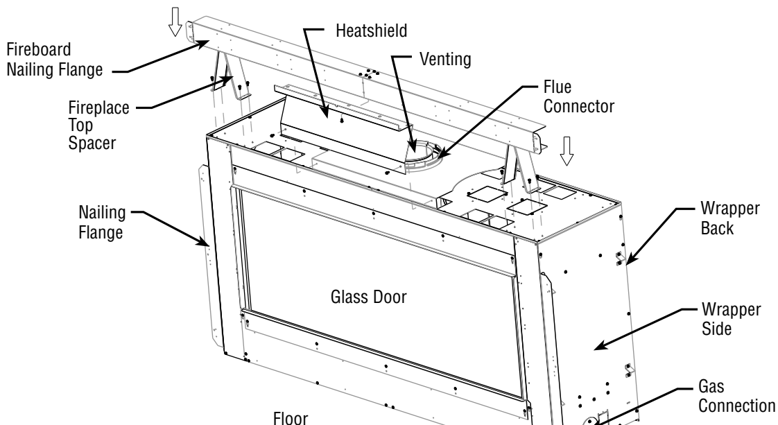
Figure 3 - Standoff Installation and Clearance to Combustibles
