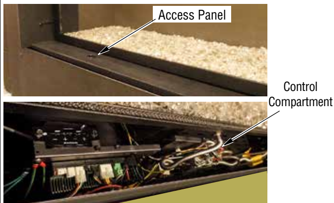
Figure 43 - Accessing The Control Compartment
