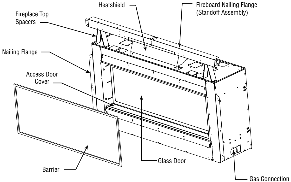
Figure 1 - Component Overview
