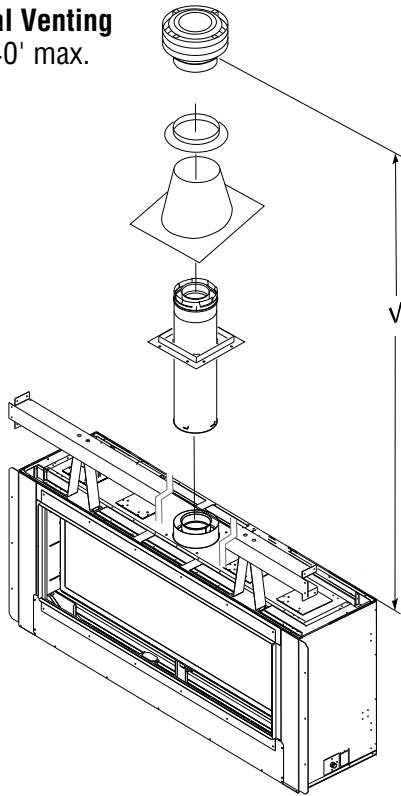
Figure 26 - Vertical Venting Configuration
