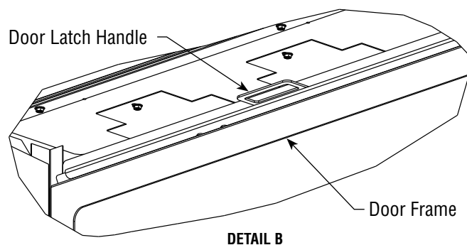
Figure 32 - Removing/Replace Glass Door
