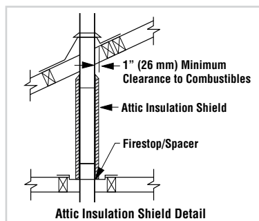
Figure 22 - Installing Firestop
