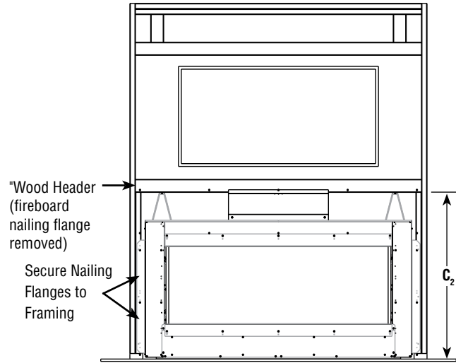
Figure 7 - Fireplace Framing Dimensions for Recessed Wall Pocket TV Installation One Sided & See-Thru Application
