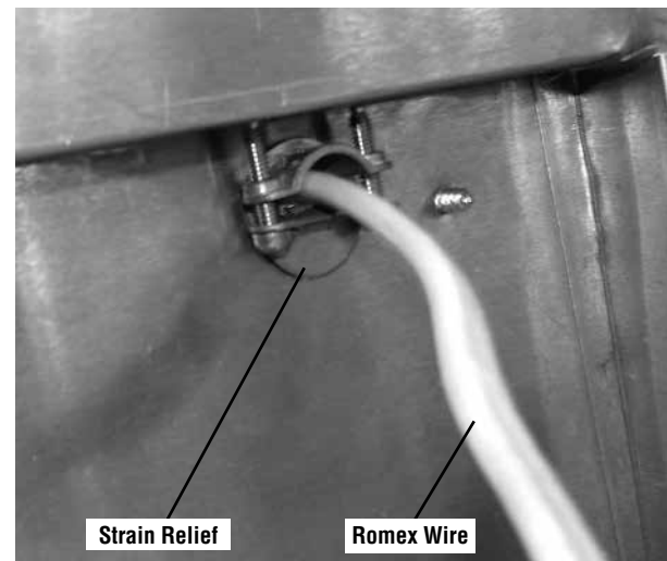
Figure 32 - Back Of Termination
