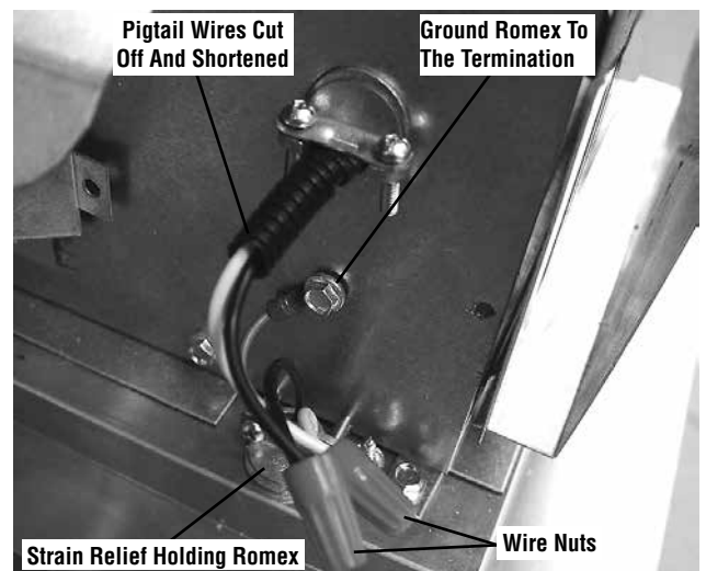
Figure 33 - Junction Box Cover Removed
