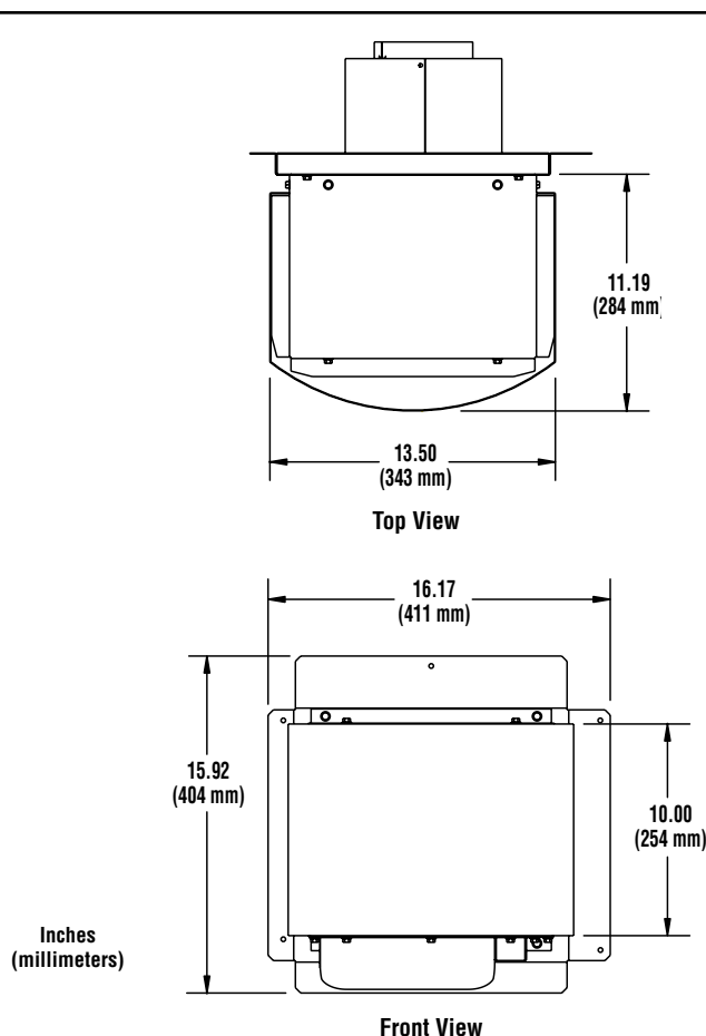
Figure 61 - Power Vent Termination Specifications
