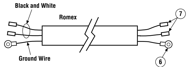
Figure 31 - Romex
