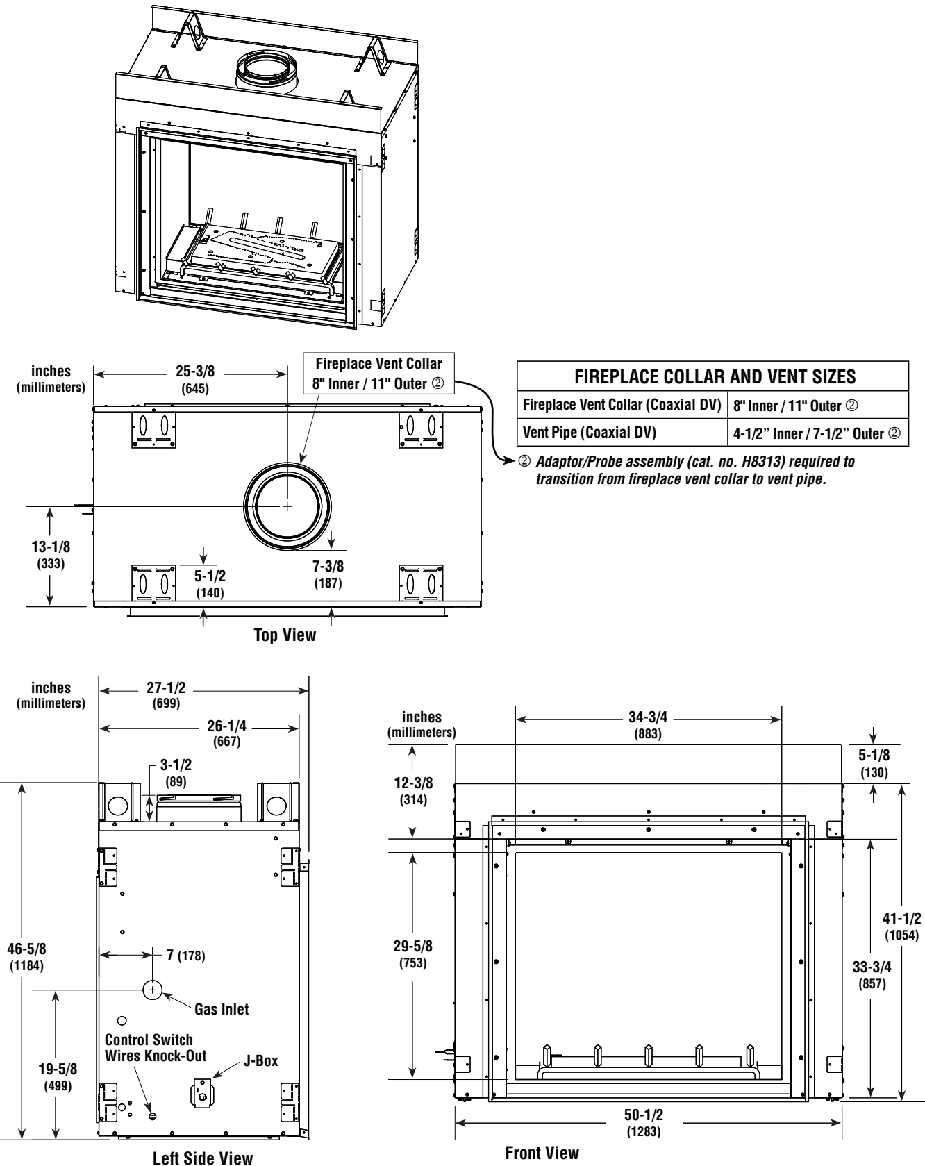
Fireplace Dimensions (shown with Outdoor Kit installed)
