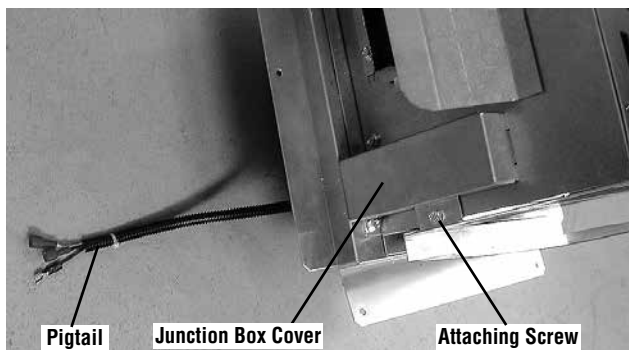
Figure 30 - Bottom of Termination
