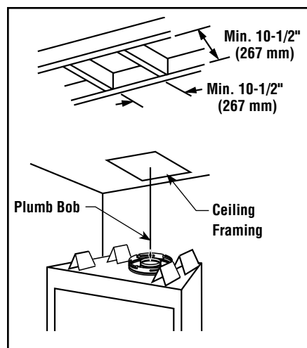
Figure 17 - Ceiling Opening Framing
