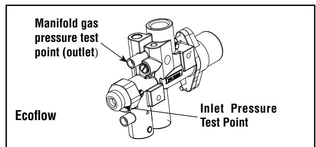
Figure 3 - MANIFOLD Outlet Gas Pressure Test Point
