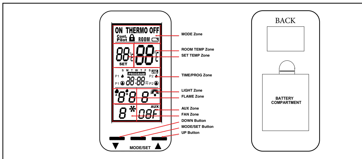
Figure 13 - Remote Control
