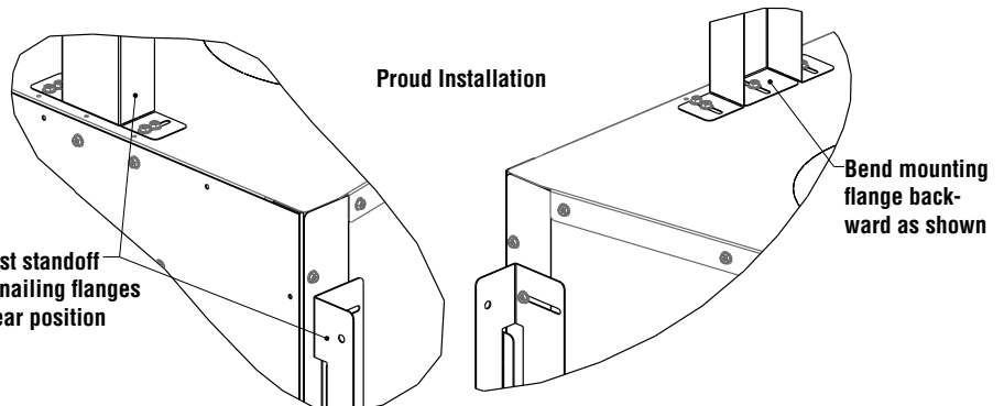
DETAIL A
