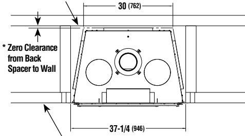
Outside Chase Rough Framing Face (unfinished shown)
