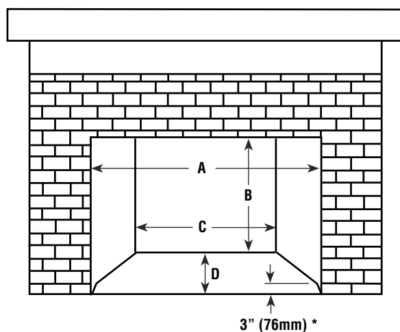
Figure 3 - Dimensions minimums de foyer requises
