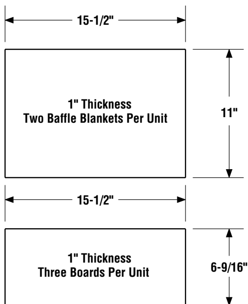
Figure 16b - Baffle Insulation Parts
