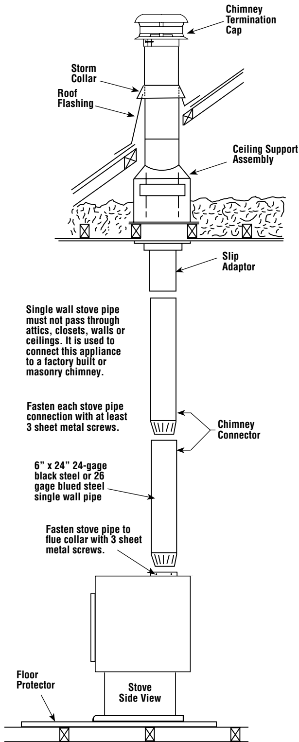
Figure 6 - Typical Installation
